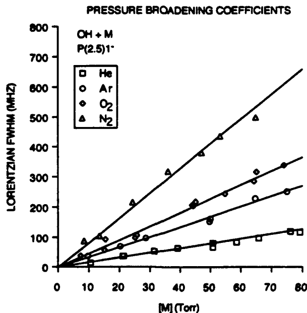
Fig. 8. Pressure broadening results for the P(2.5)1' transition in OH( v=1\leftarrow 0 ) in the presence of N 2 , O 2 , Ar and He buffer gas
